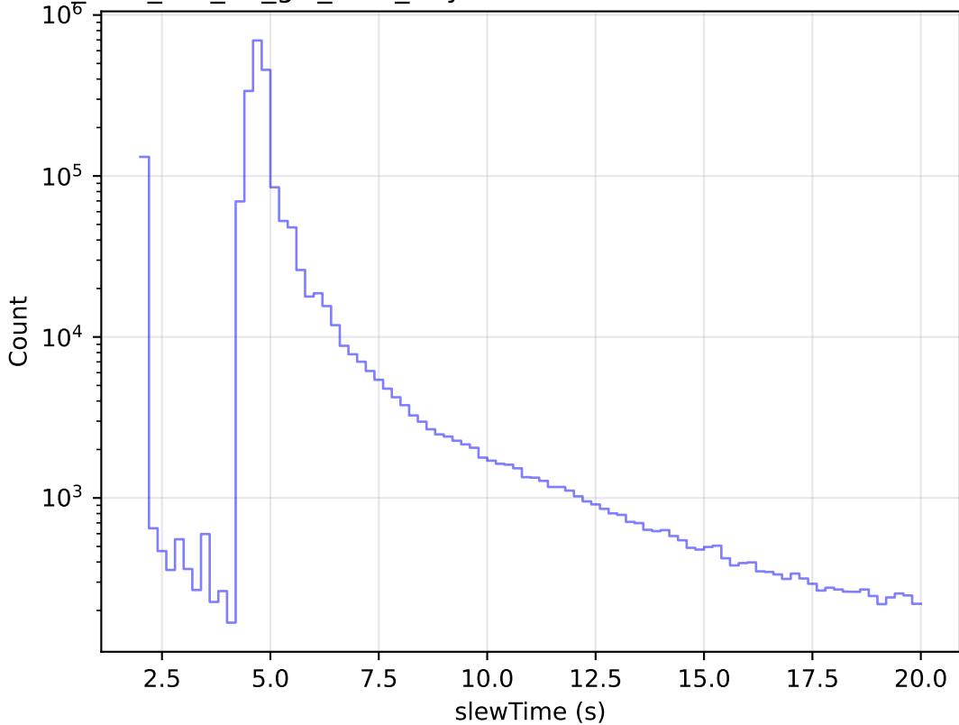
too_elab_r64_d2_giz_v3.4_10yrs All visits: Zoom Slew Time Histogram
