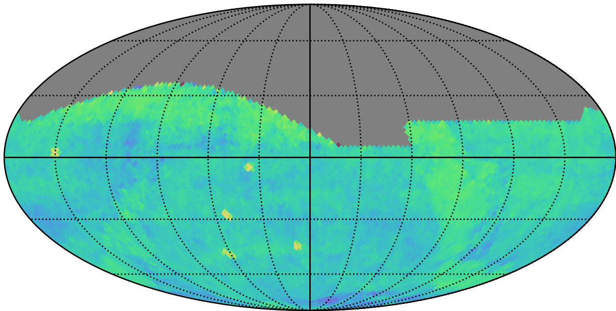
too_elab_r64_d2_giz_v3.4_10yrs (g or r or i): PairFraction
