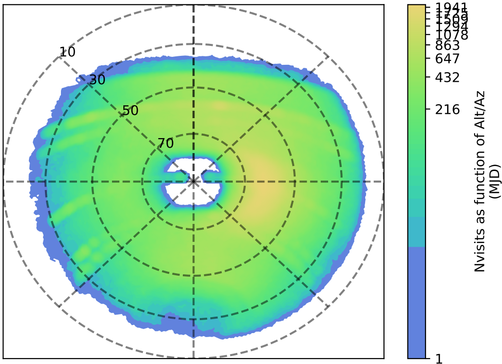
too_elab_r64_d2_giz_v3.4_10yrs y: Nvisits as function of Alt/Az
