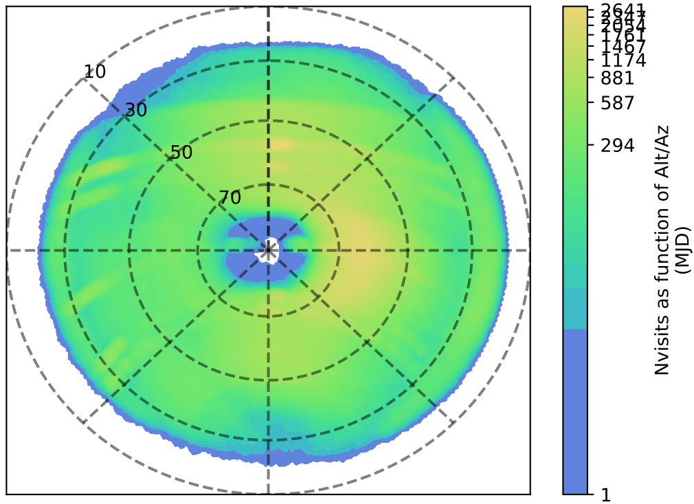
too_elab_r64_d2_giz_v3.4_10yrs i: Nvisits as function of Alt/Az
