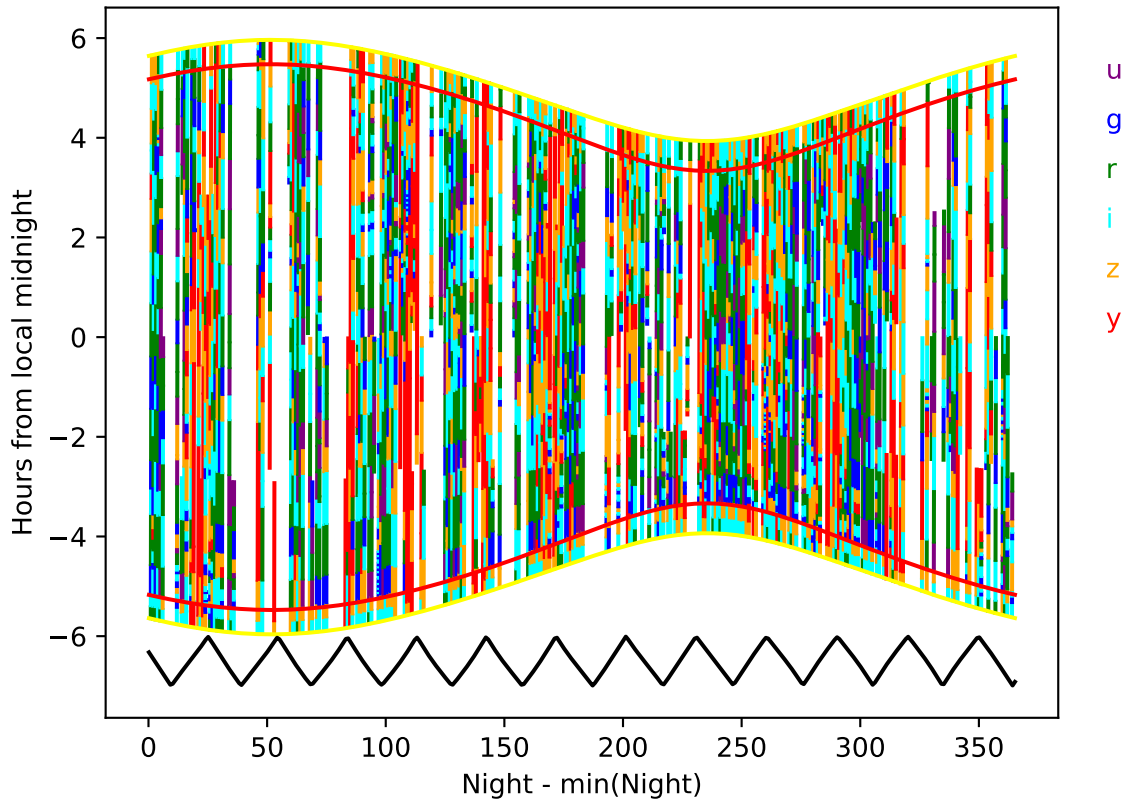
too_elab_r64_d2_giz_v3.4_10yrs year 7-8: Hourglass
