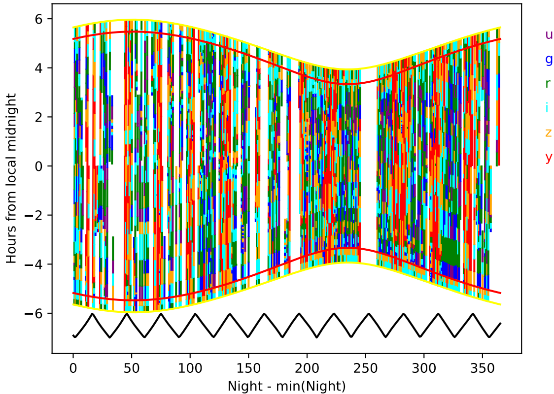
too_elab_r64_d2_giz_v3.4_10yrs year 5-6: Hourglass
