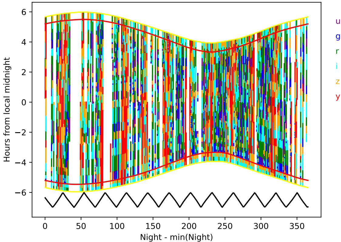
too_elab_r64_d2_giz_v3.4_10yrs year 4-5: Hourglass
