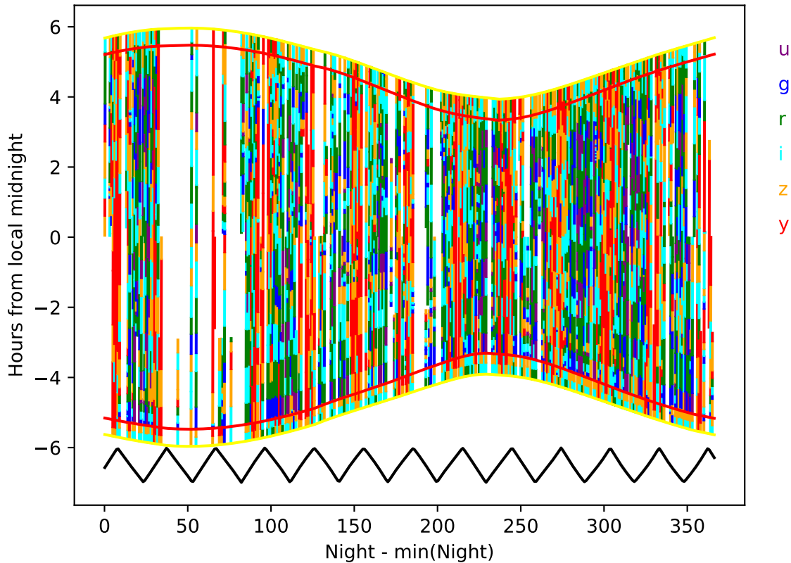
too_elab_r64_d2_giz_v3.4_10yrs year 3-4: Hourglass
