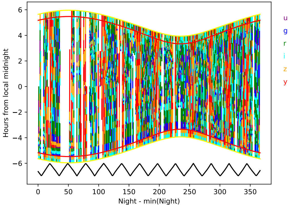
too_elab_r64_d2_giz_v3.4_10yrs year 2-3: Hourglass
