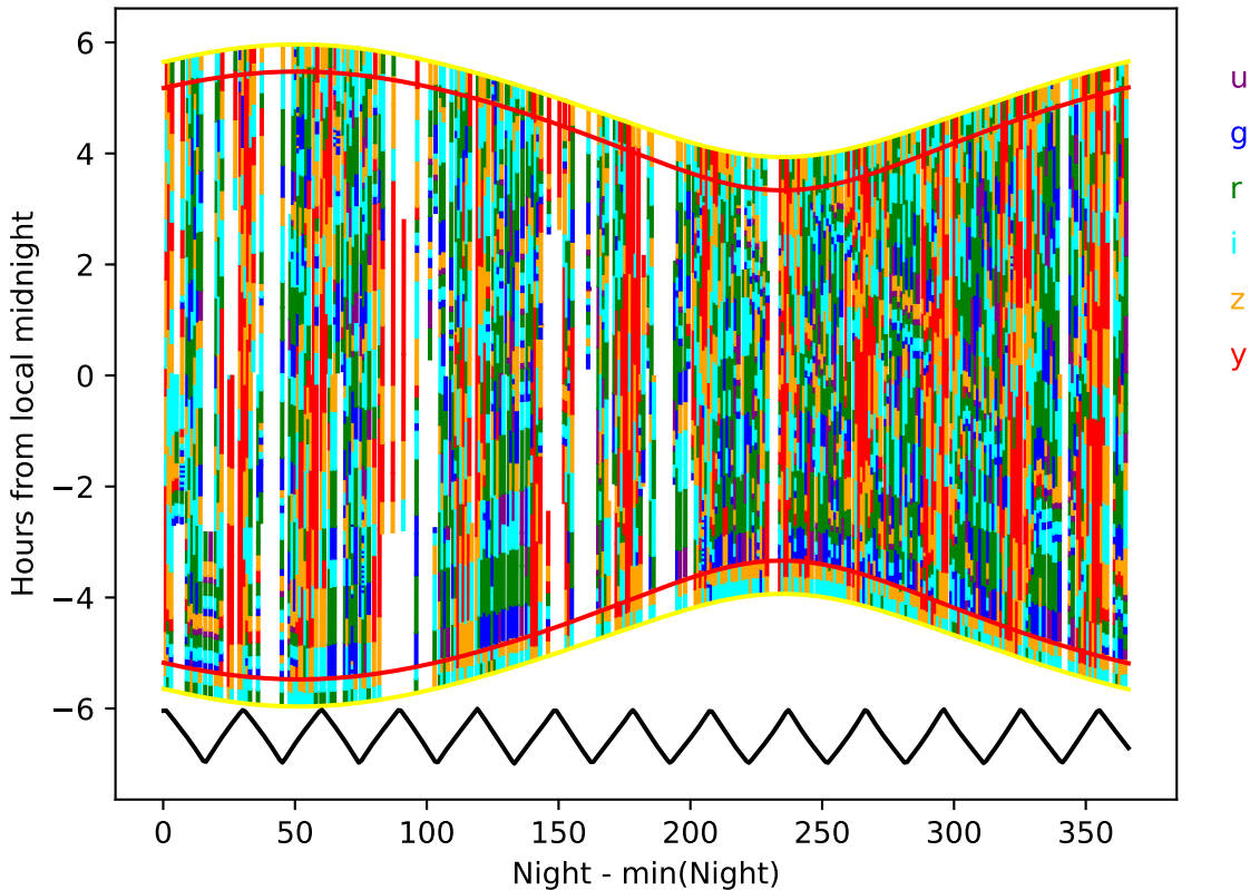
too_elab_r64_d2_giz_v3.4_10yrs year 1-2: Hourglass
