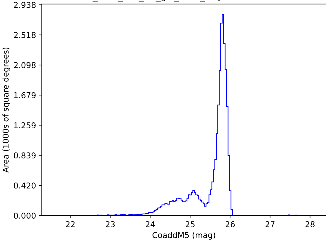
too_elab_r64_d2_giz_v3.4_10yrs z: CoaddM5
