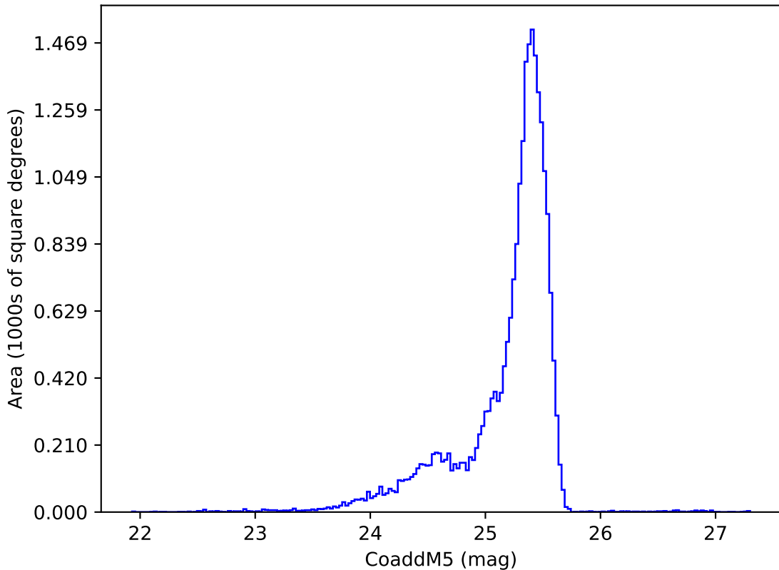
too_elab_r64_d2_giz_v3.4_10yrs u: CoaddM5
