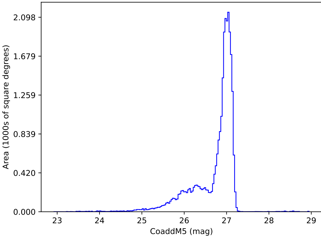
too_elab_r64_d2_giz_v3.4_10yrs r: CoaddM5
