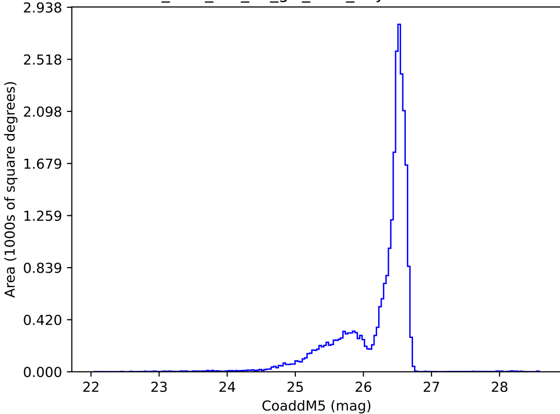
too_elab_r64_d2_giz_v3.4_10yrs i: CoaddM5
