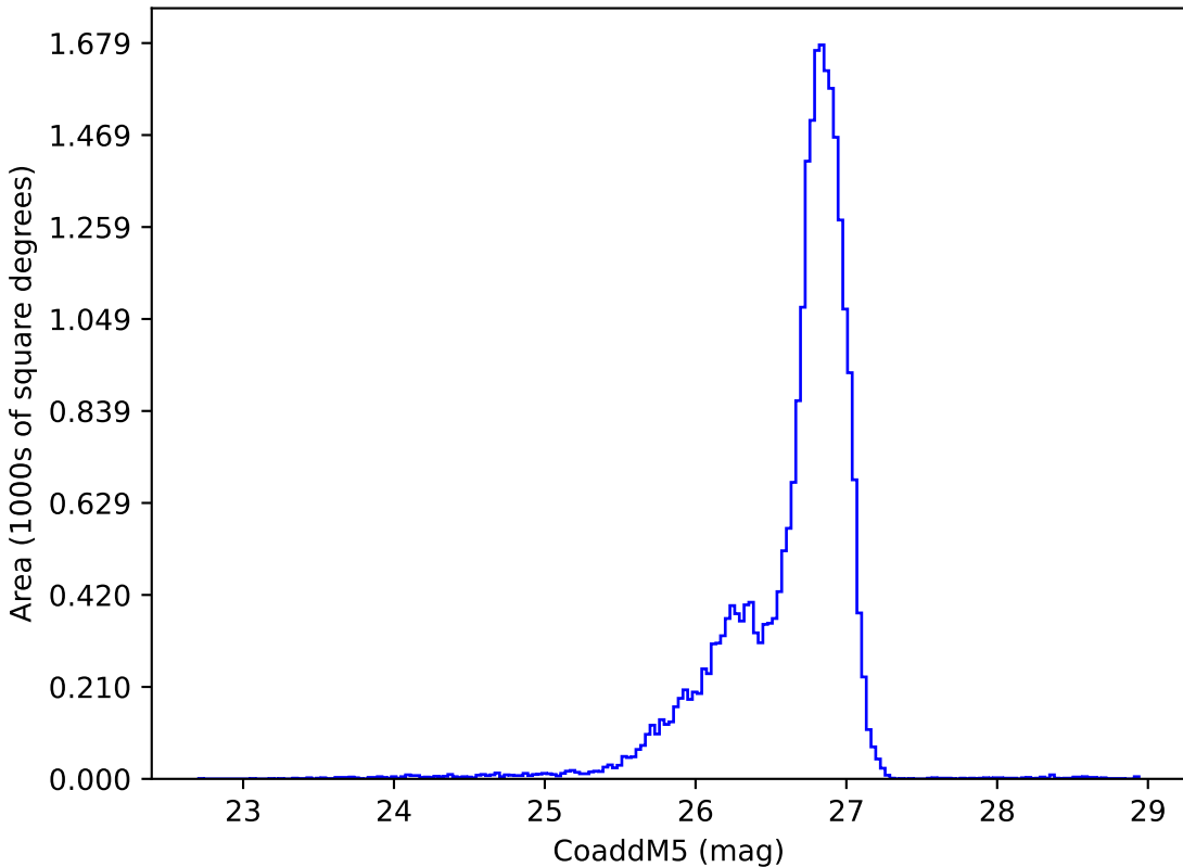
too_elab_r64_d2_giz_v3.4_10yrs g: CoaddM5
