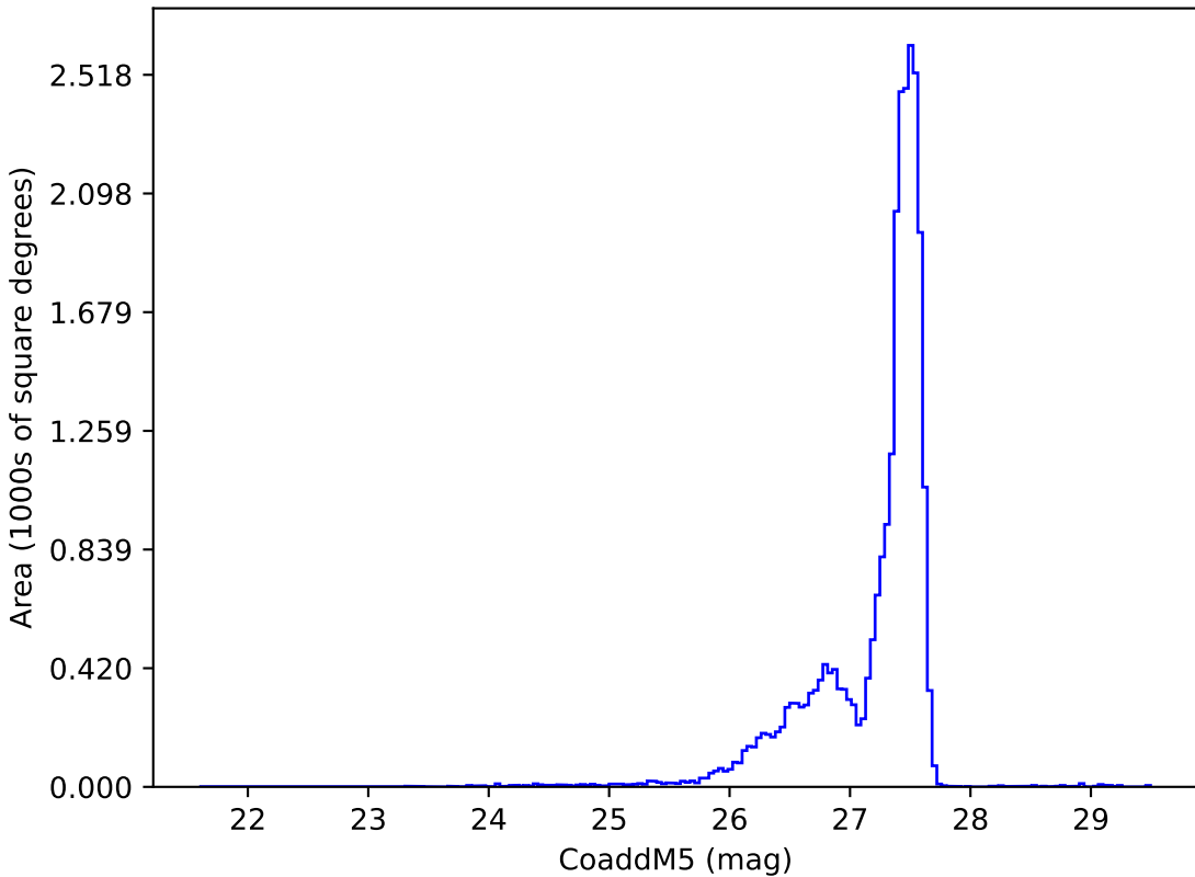
too_elab_r64_d2_giz_v3.4_10yrs : CoaddM5
