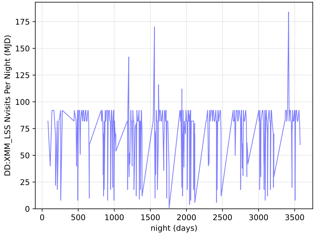
too_elab_r64_d2_giz_v3.4_10yrs all bands: DD:XMM_LSS Nvisits Per Night
