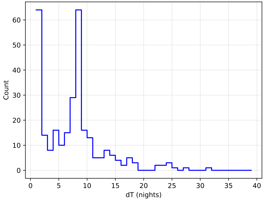
too_elab_r64_d2_giz_v3.4_10yrs all bands: DD:XMM_LSS Delta Nights Histogram
