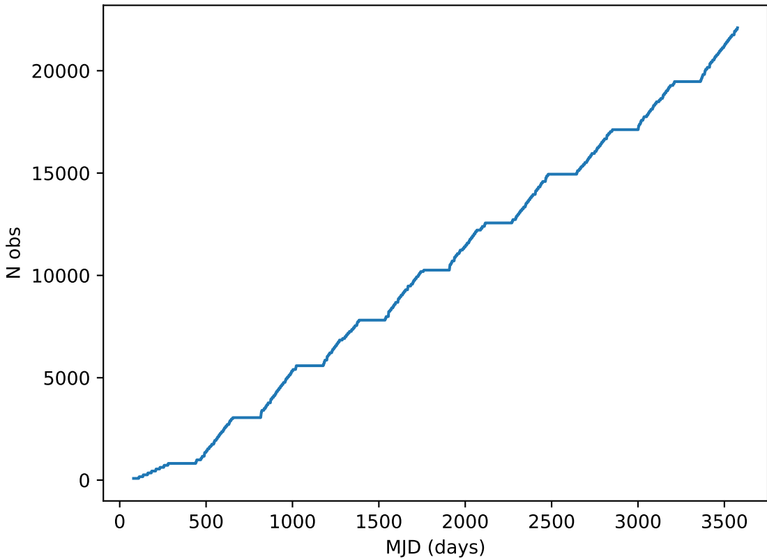
too_elab_r64_d2_giz_v3.4_10yrs all bands: DD:XMM_LSS Cumulative NVisits
