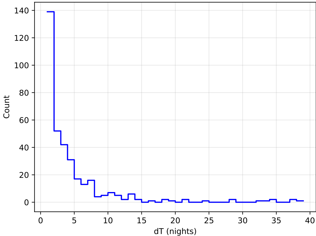
too_elab_r64_d2_giz_v3.4_10yrs all bands: DD:WFD Delta Nights Histogram
