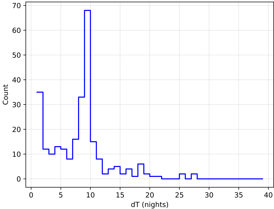
too_elab_r64_d2_giz_v3.4_10yrs all bands: DD:ELAISS1 Delta Nights Histogram
