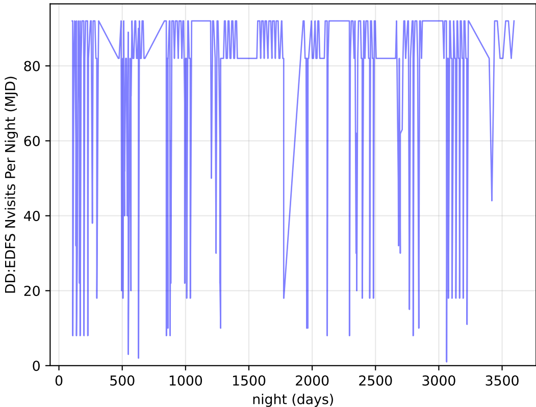
too_elab_r64_d2_giz_v3.4_10yrs all bands: DD:EDFS Nvisits Per Night
