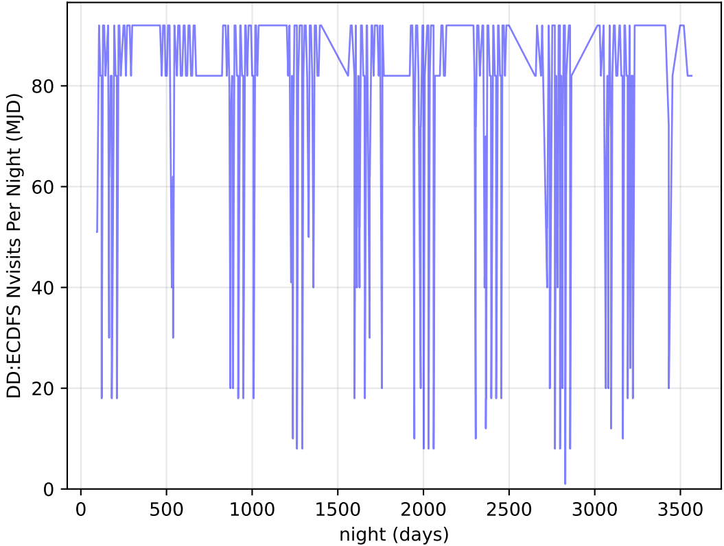
too_elab_r64_d2_giz_v3.4_10yrs all bands: DD:ECDFS Nvisits Per Night
