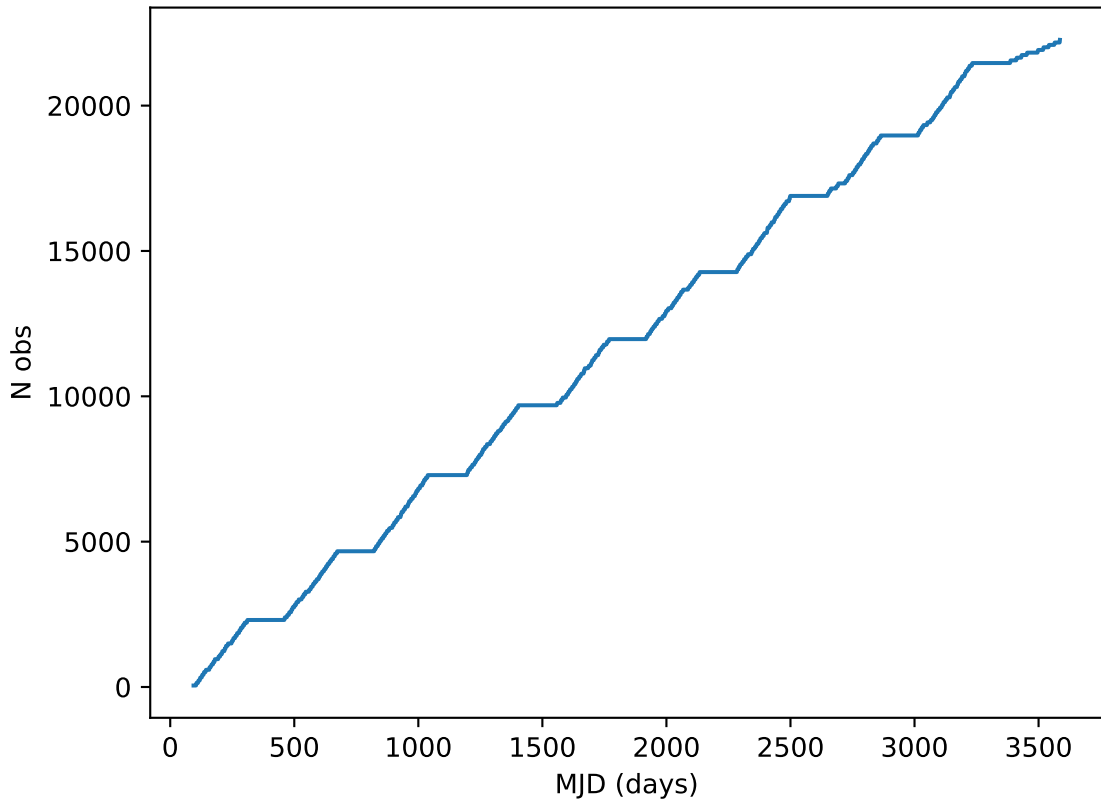
too_elab_r64_d2_giz_v3.4_10yrs all bands: DD:ECDFS Cumulative NVisits
