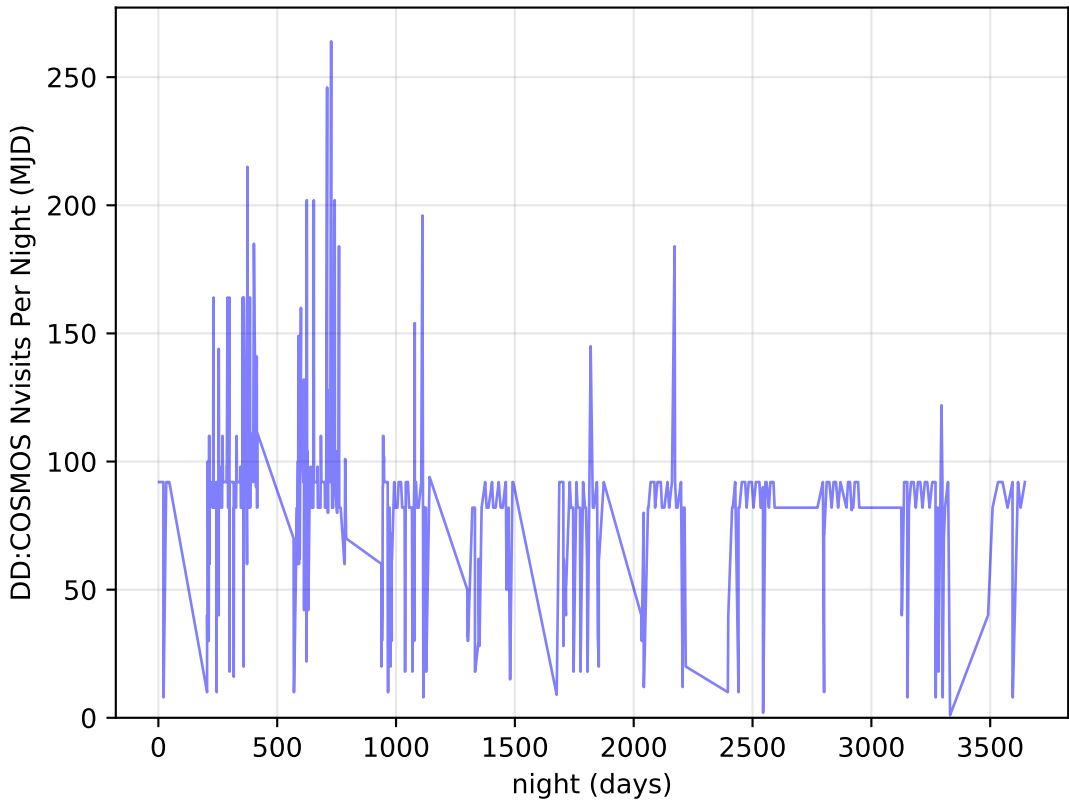
too_elab_r64_d2_giz_v3.4_10yrs all bands: DD: COSMOS Nvisits Per Night
