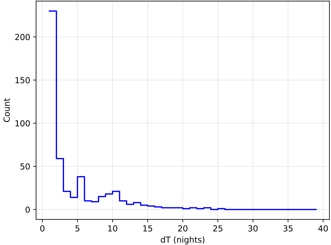
too_elab_r64_d2_giz_v3.4_10yrs all bands: DD: COSMOS Delta Nights Histogram
