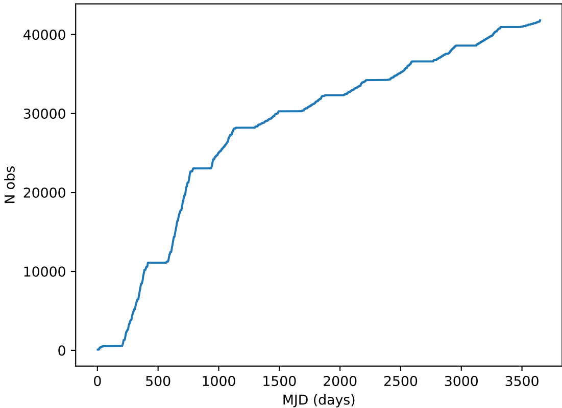
too_elab_r64_d2_giz_v3.4_10yrs all bands: DD:COSMOS Cumulative NVisits
