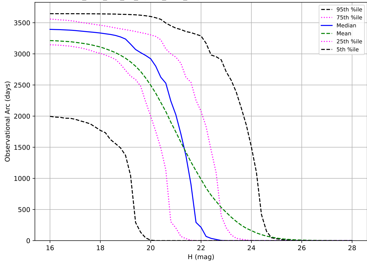
too_elab_r32_d3_ugrizy_v3.4_10yrs: Observational Arc Length PHA
