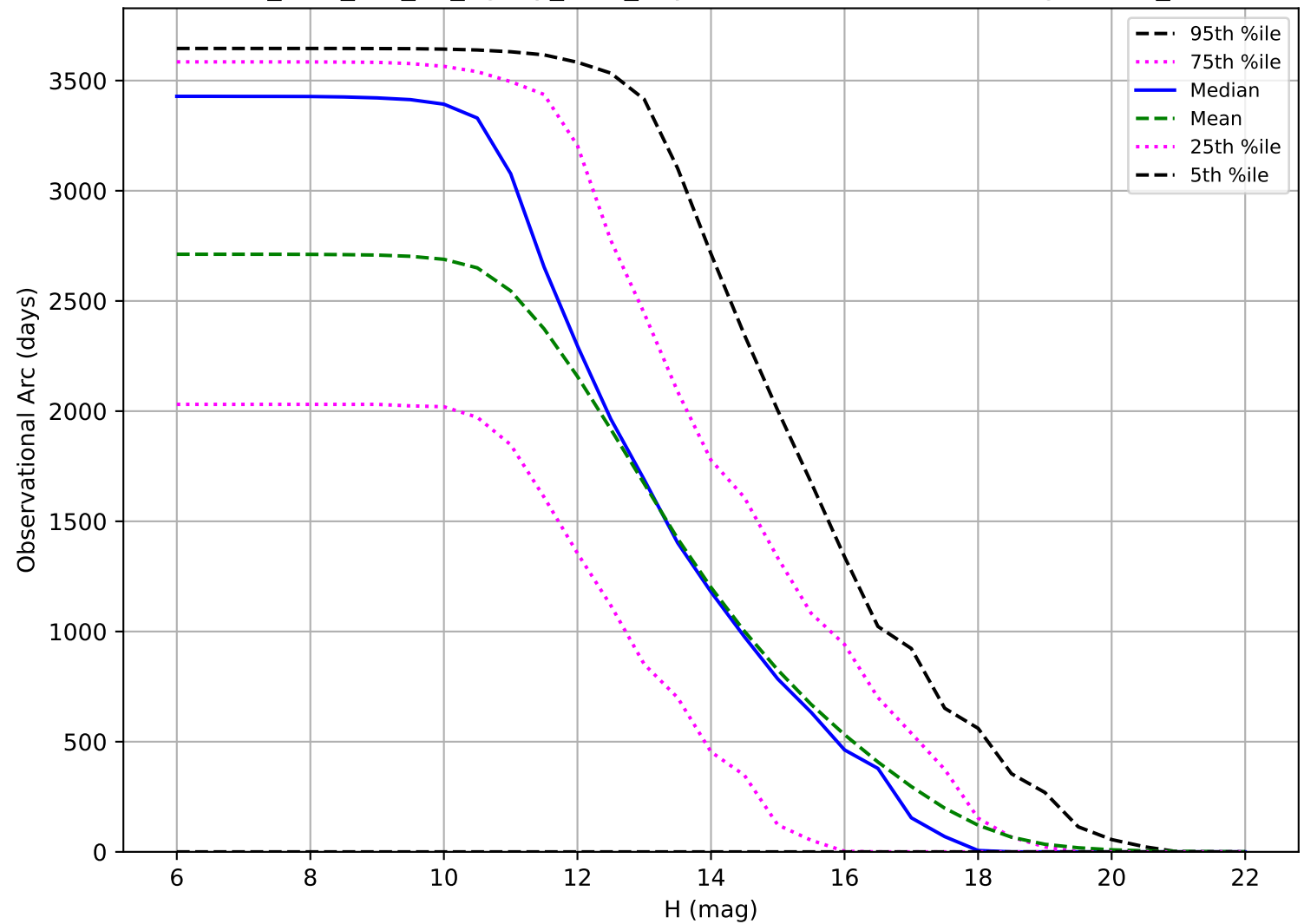
too_elab_r32_d3_ugrizy_v3.4_10yrs: Observational Arc Length OCC_r5
