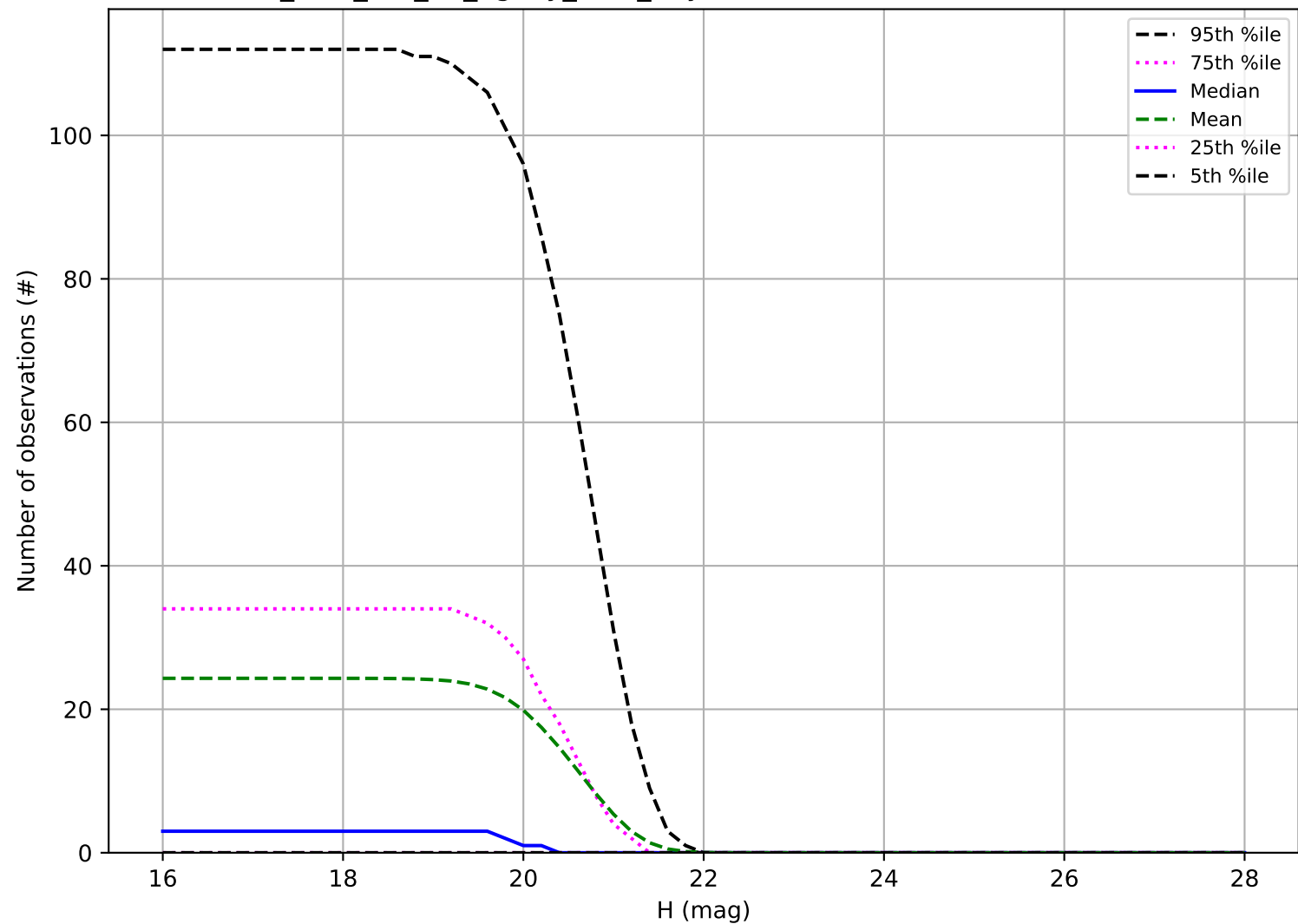
too_elab_r32_d3_ugrizy_v3.4_10yrs: Number of observations Vatira
