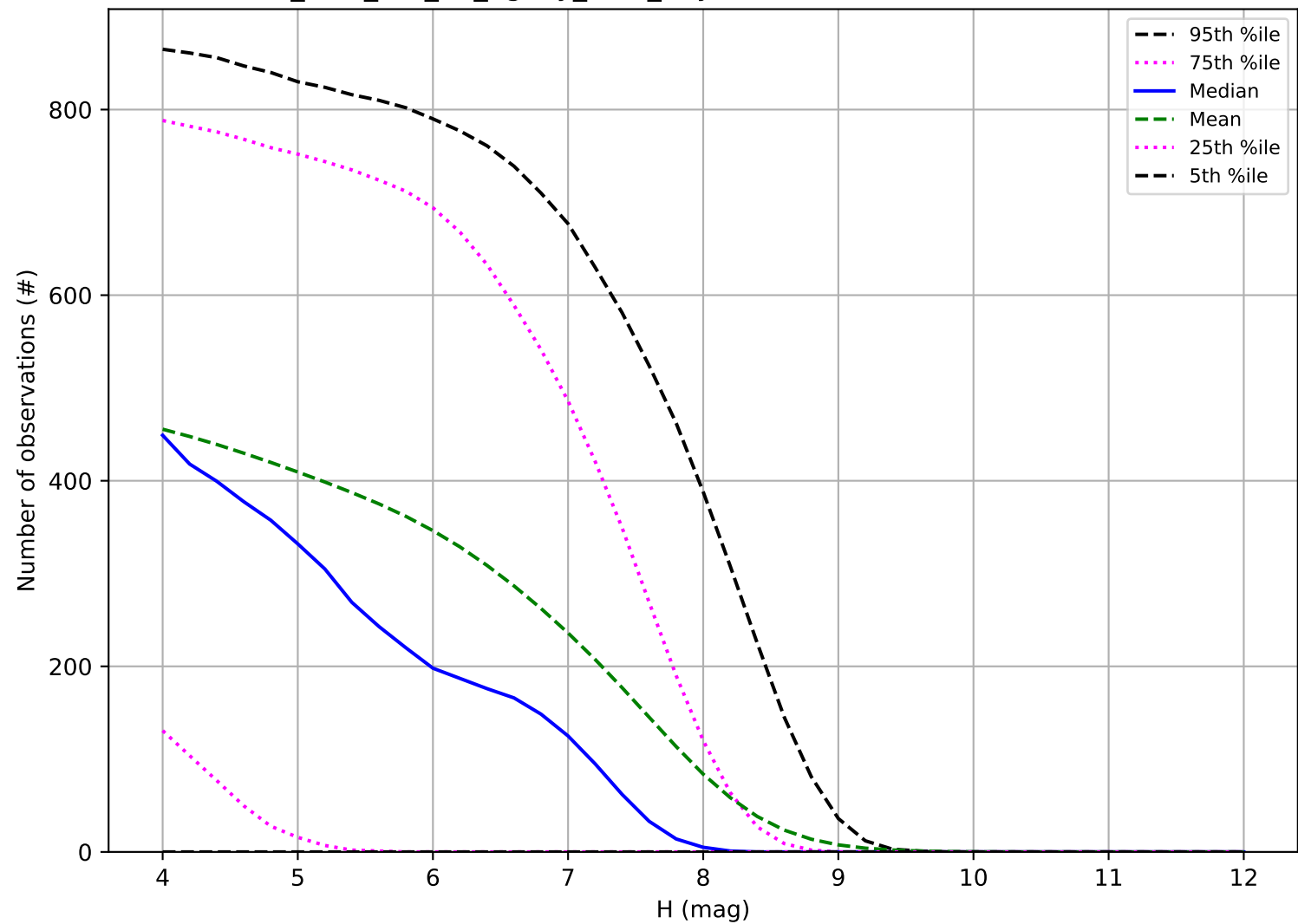
too_elab_r32_d3_ugrizy_v3.4_10yrs: Number of observations TNO
