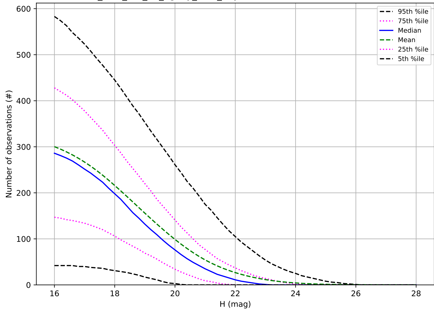
too_elab_r32_d3_ugrizy_v3.4_10yrs: Number of observations PHA
