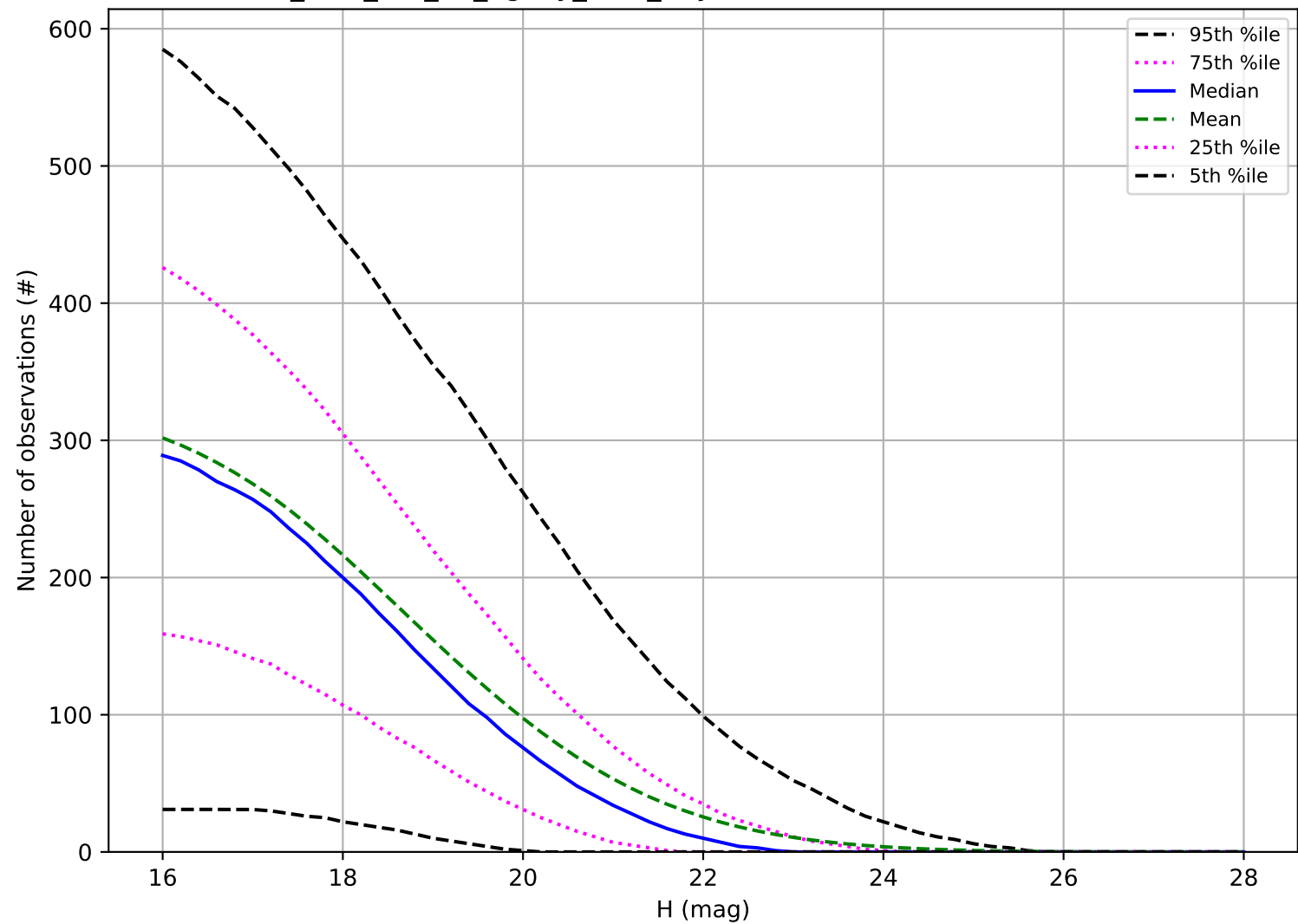
too_elab_r32_d3_ugrizy_v3.4_10yrs: Number of observations NEO
