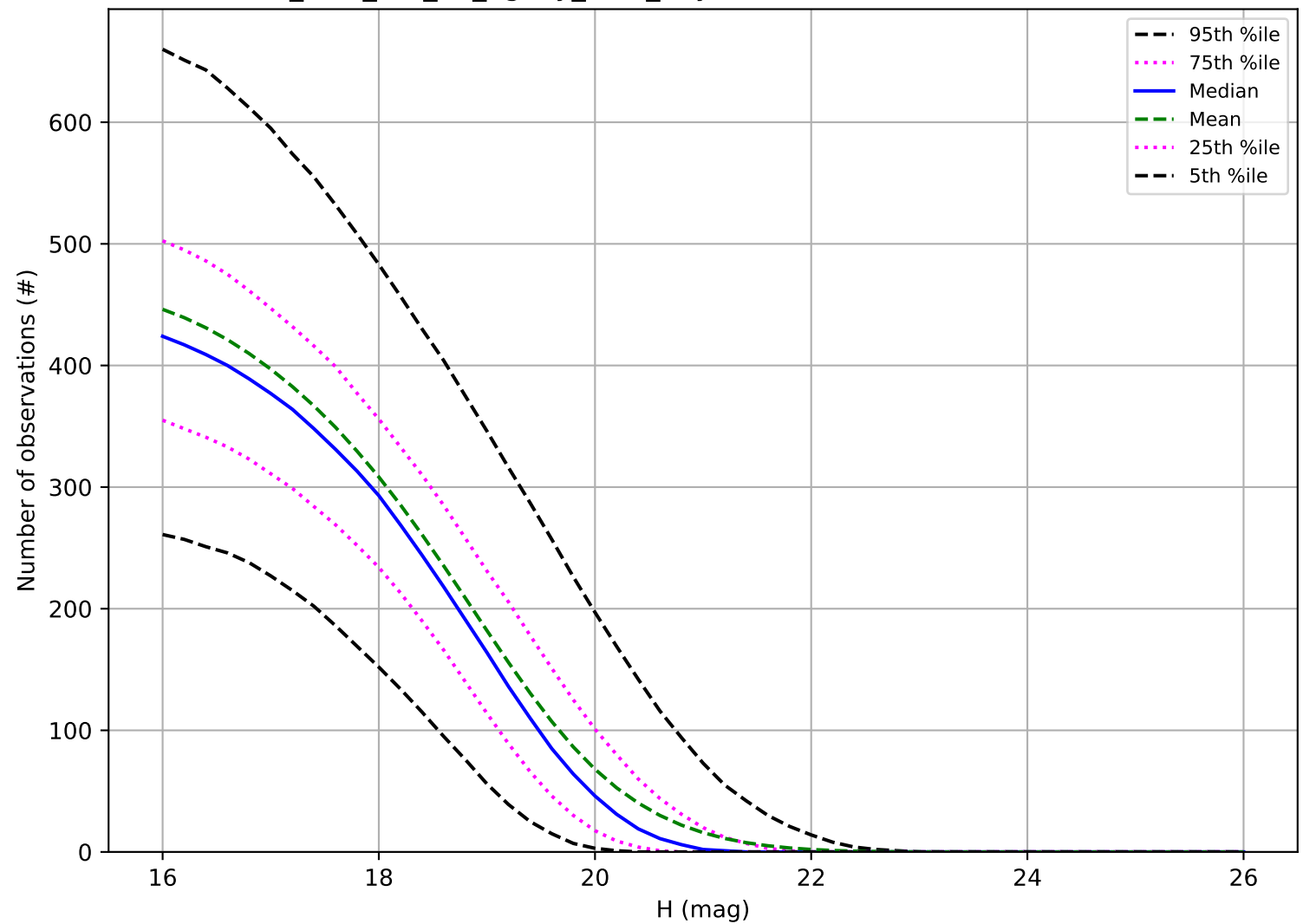
too_elab_r32_d3_ugrizy_v3.4_10yrs: Number of observations MBA
