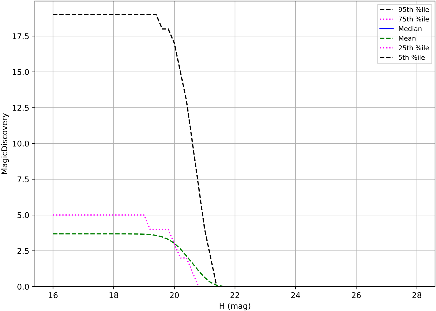
too_elab_r32_d3_ugrizy_v3.4_10yrs: Vatira 6 detections in 60 nights detection loss
