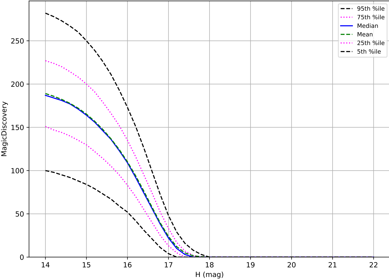
too_elab_r32_d3_ugrizy_v3.4_10yrs: Trojan 6 detections in 60 nights detection loss
