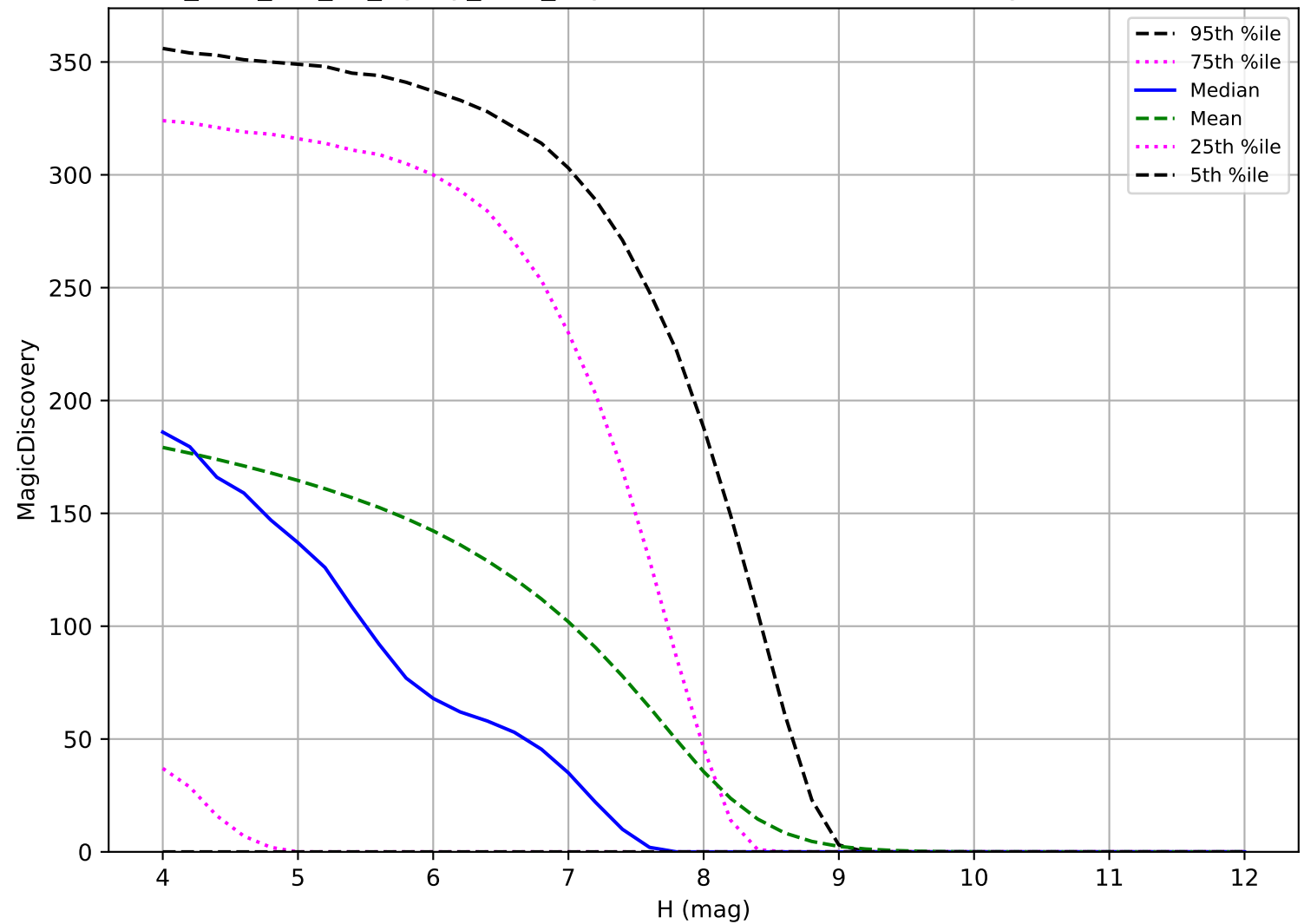
too_elab_r32_d3_ugrizy_v3.4_10yrs: TNO 6 detections in 60 nights detection loss
