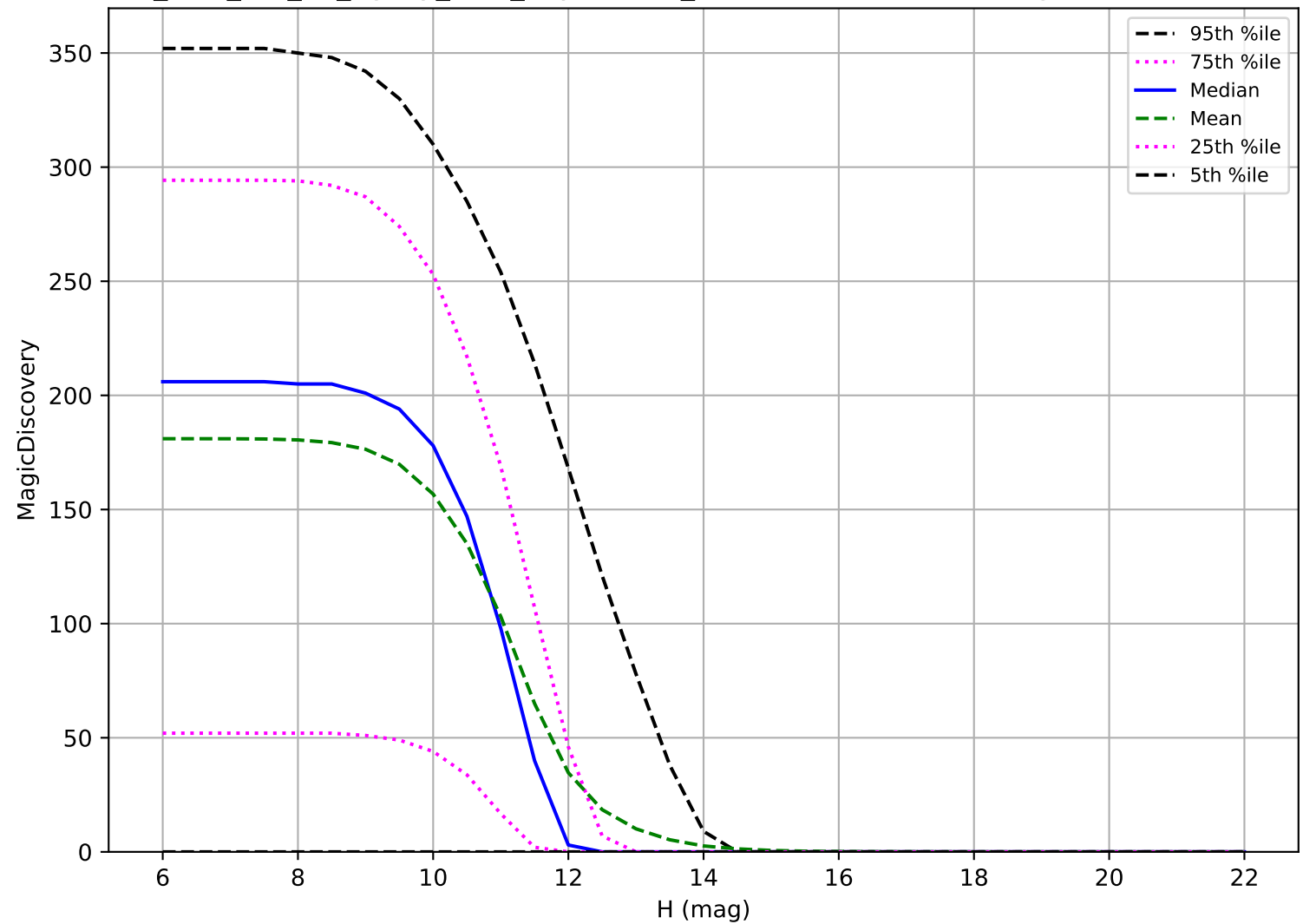
too_elab_r32_d3_ugrizy_v3.4_10yrs: OCC_r20 6 detections in 60 nights detection loss
