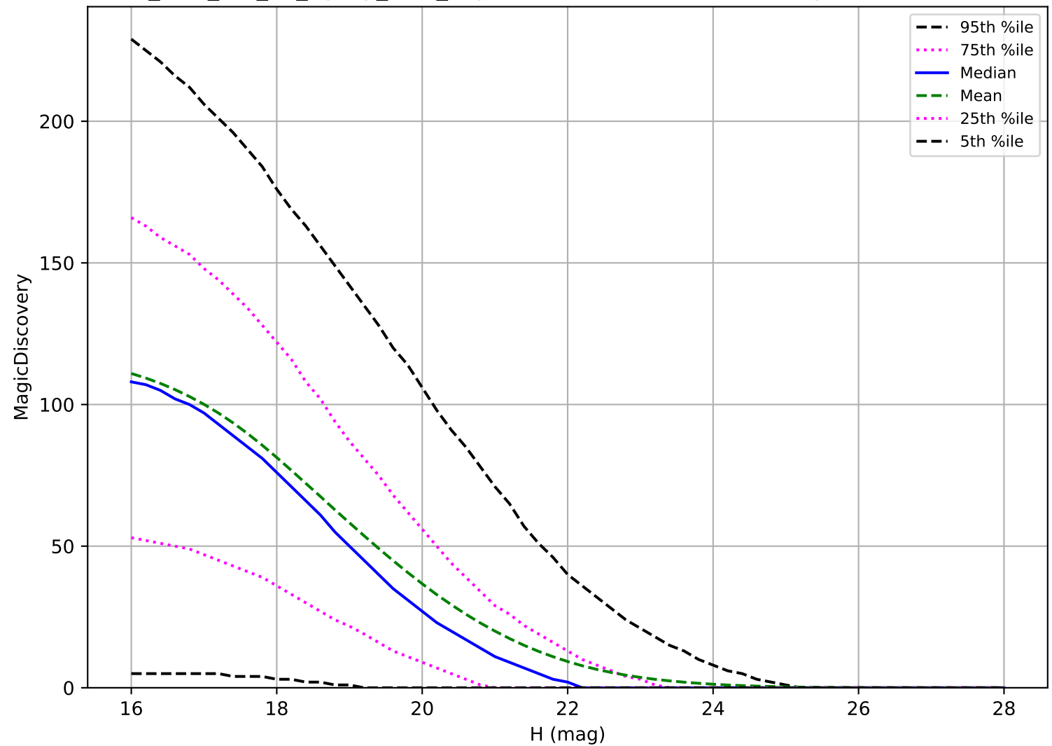
too_elab_r32_d3_ugrizy_v3.4_10yrs: NEO 6 detections in 60 nights detection loss
