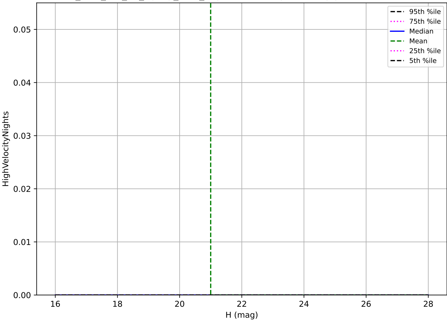
too_elab_r32_d3_ugrizy_v3.4_10yrs: Vatira High velocity pair detection loss
