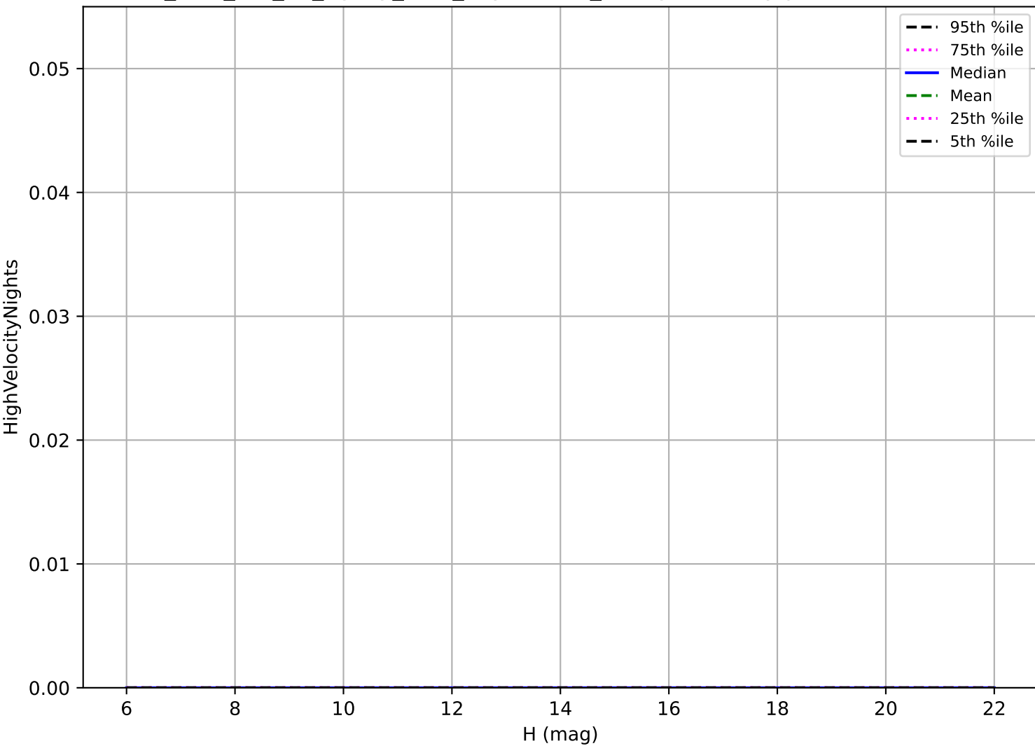
too_elab_r32_d3_ugrizy_v3.4_10yrs: OCC_r5 High velocity pair detection loss
