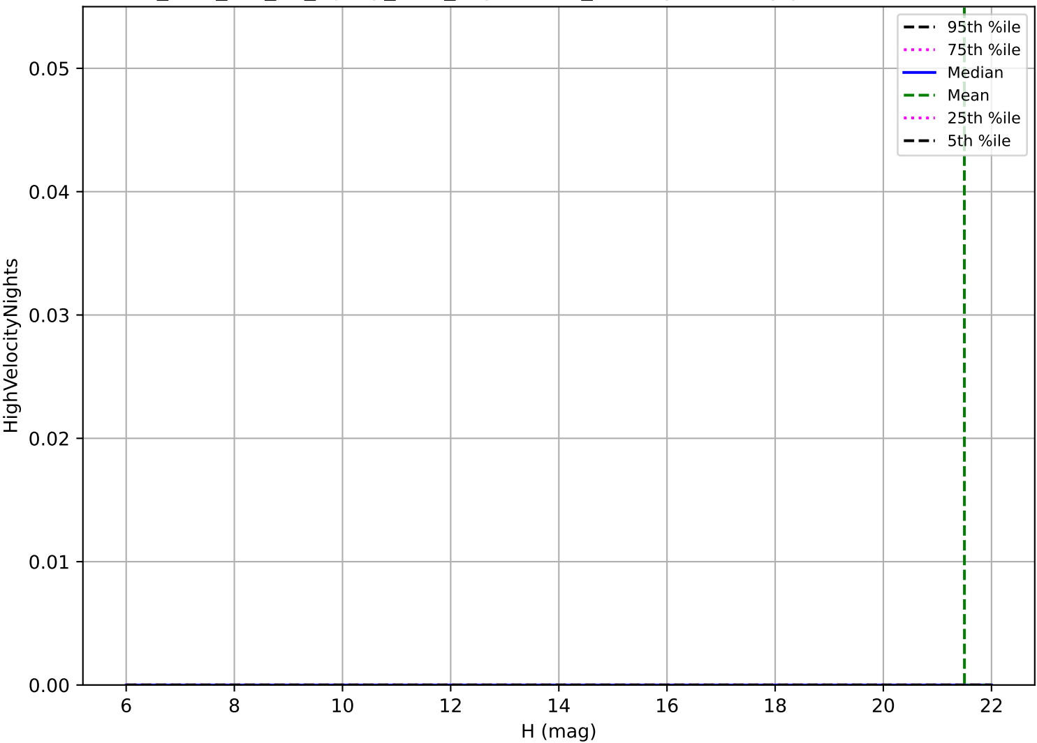
too_elab_r32_d3_ugrizy_v3.4_10yrs: OCC_r20 High velocity pair detection loss
