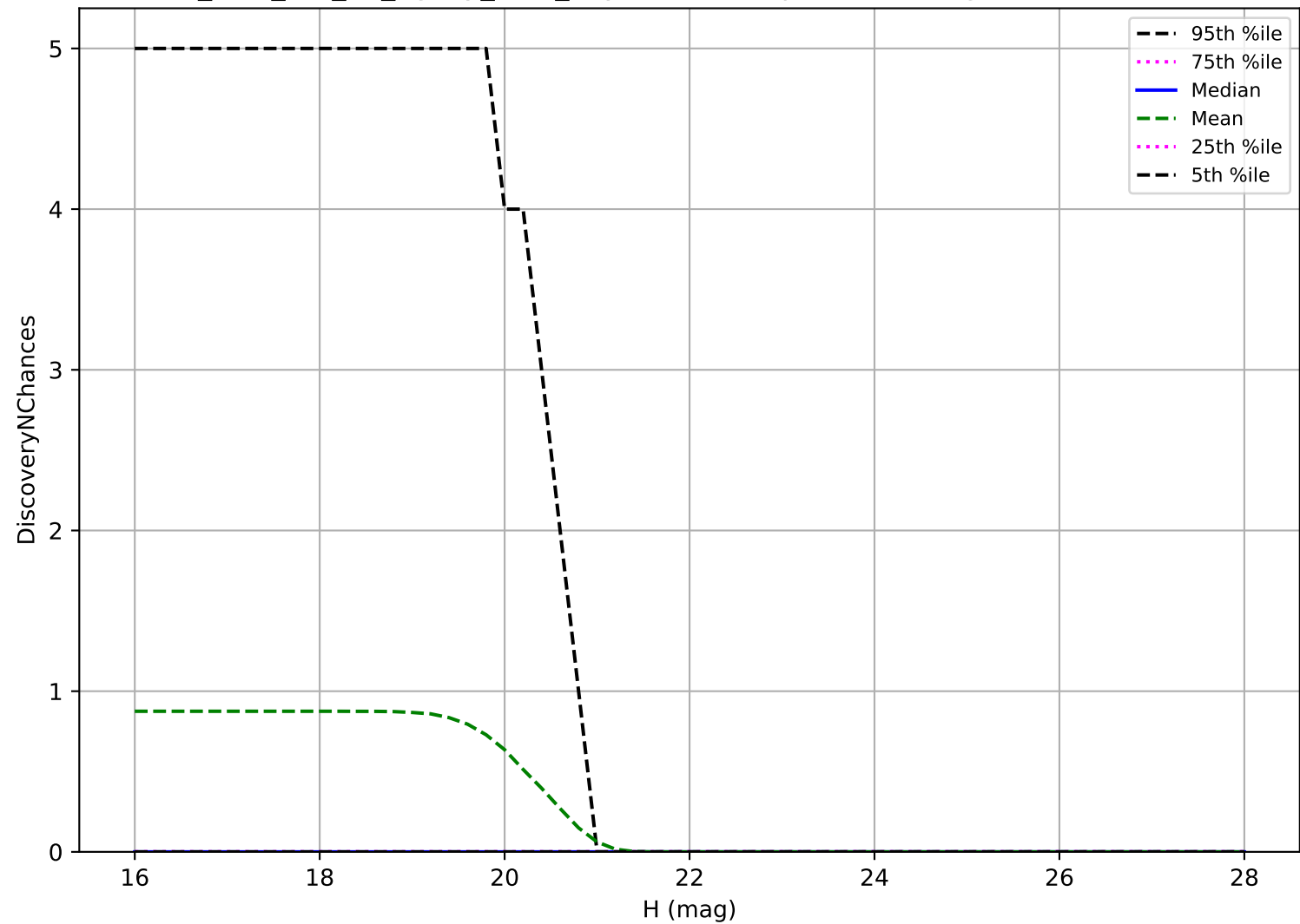
too_elab_r32_d3_ugrizy_v3.4_10yrs: Vatira 3 pairs in 15 nights detection loss
