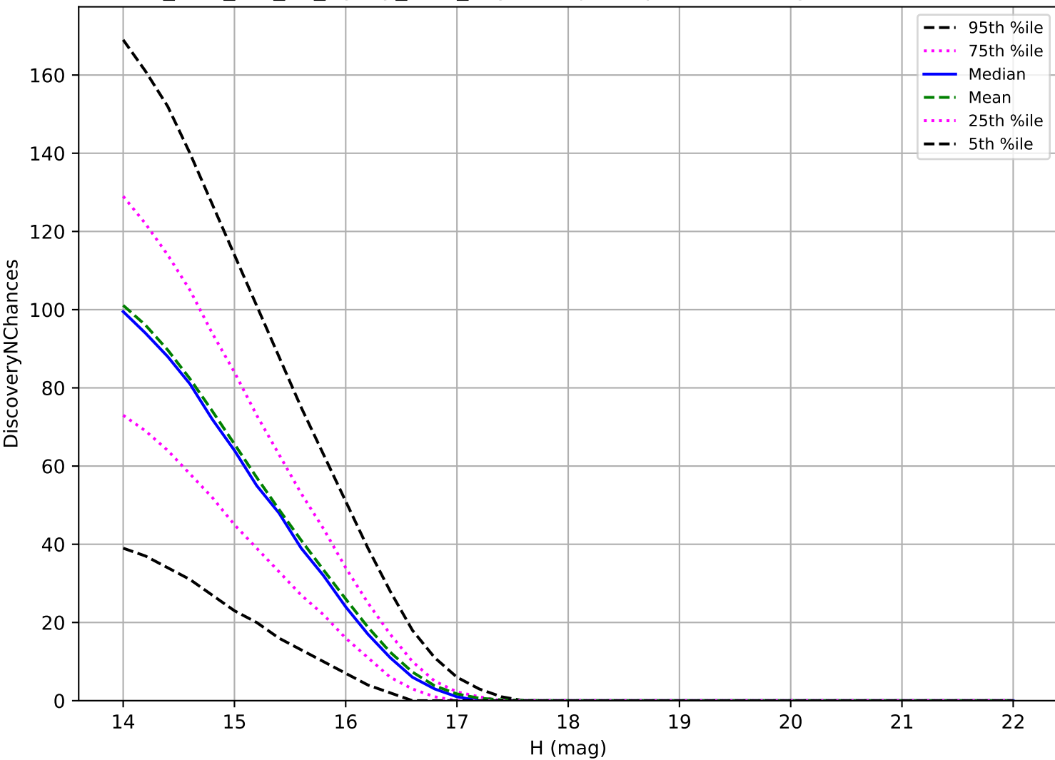
too_elab_r32_d3_ugrizy_v3.4_10yrs: Trojan 3 pairs in 15 nights detection loss
