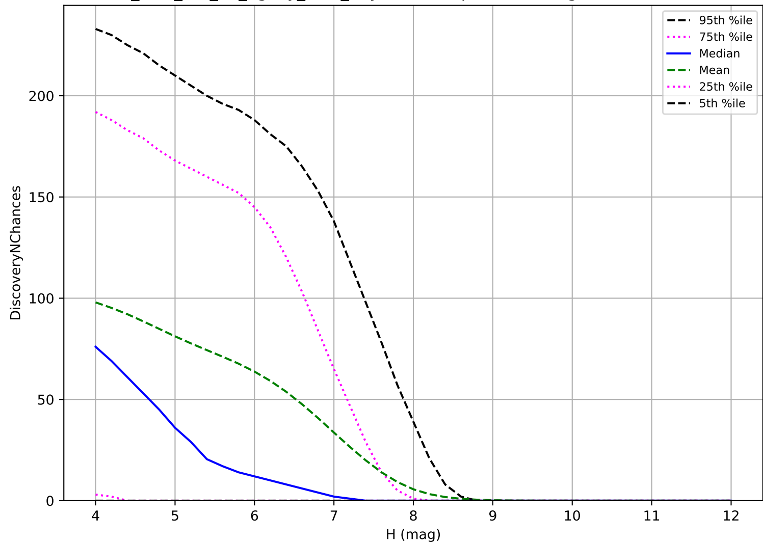
too_elab_r32_d3_ugrizy_v3.4_10yrs: TNO 3 pairs in 15 nights detection loss
