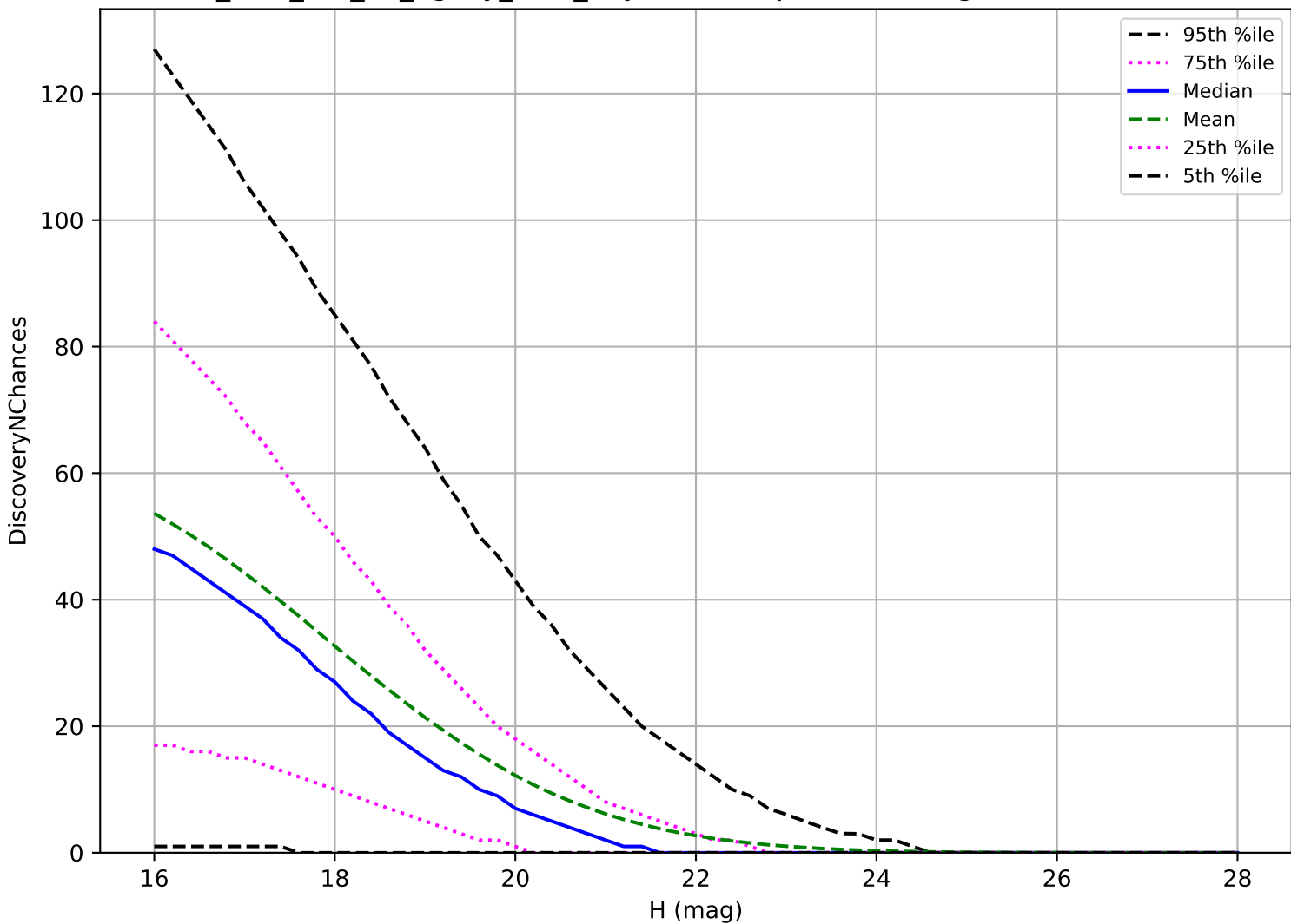
too_elab_r32_d3_ugrizy_v3.4_10yrs: PHA 3 pairs in 15 nights detection loss
