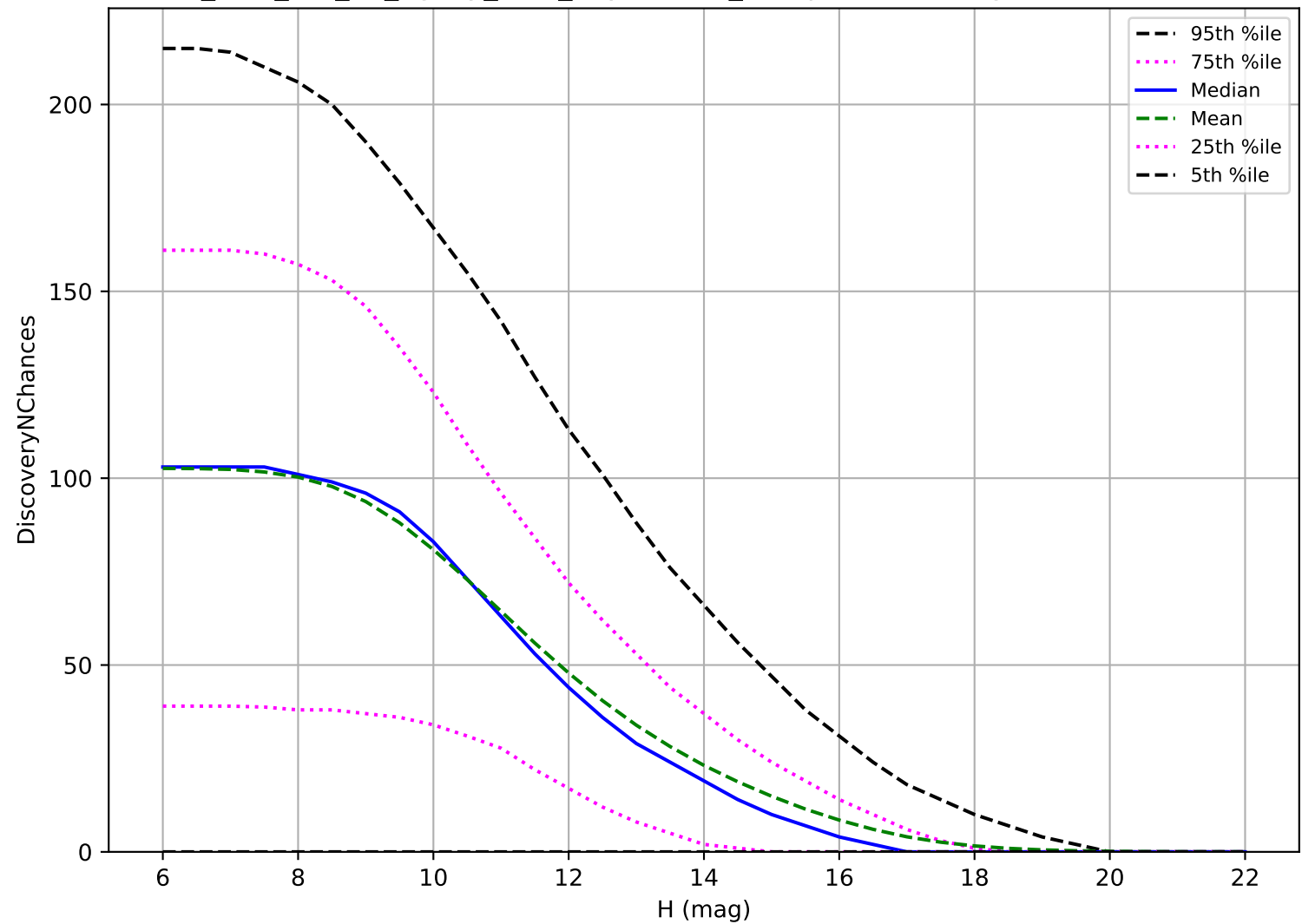
too_elab_r32_d3_ugrizy_v3.4_10yrs: OCC_r5 3 pairs in 15 nights detection loss
