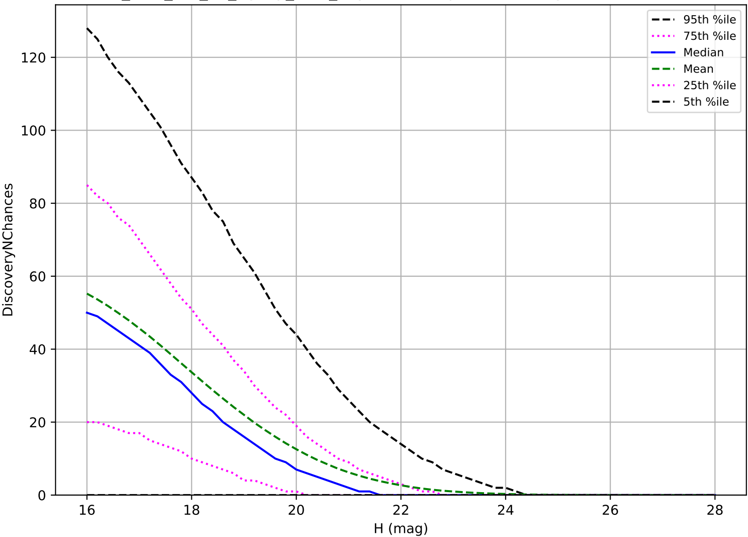
too_elab_r32_d3_ugrizy_v3.4_10yrs: NEO 3 pairs in 15 nights detection loss
