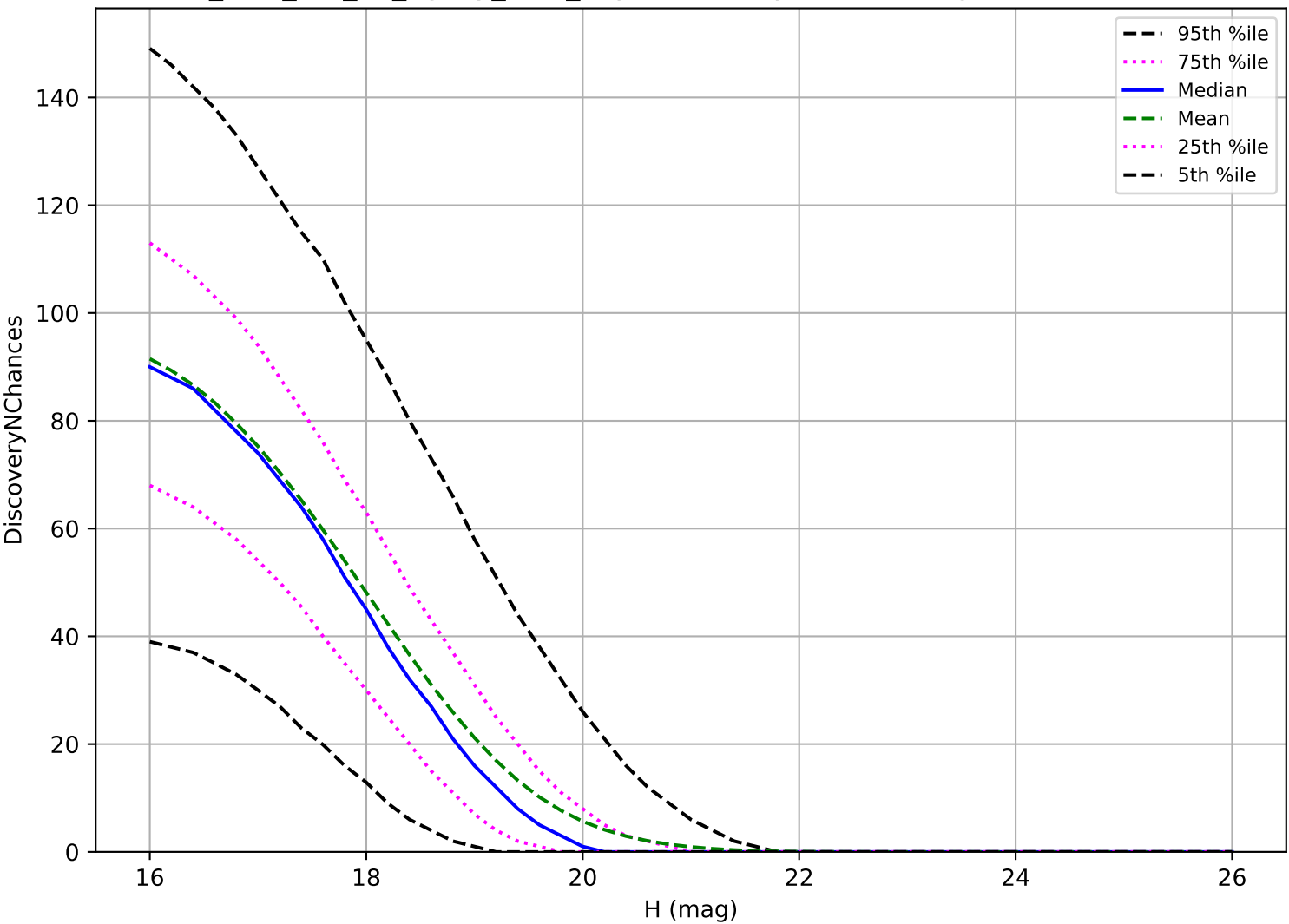
too_elab_r32_d3_ugrizy_v3.4_10yrs: MBA 3 pairs in 15 nights detection loss
