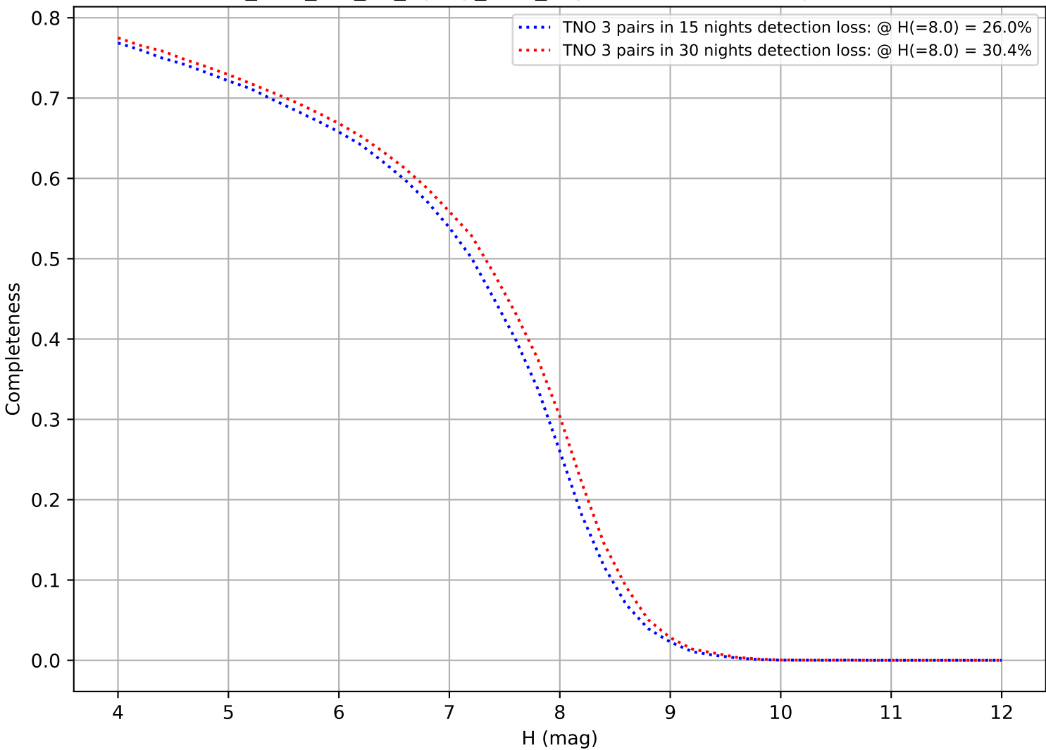
too_elab_r32_d3_ugrizy_v3.4_10yrs: DifferentialCompleteness
